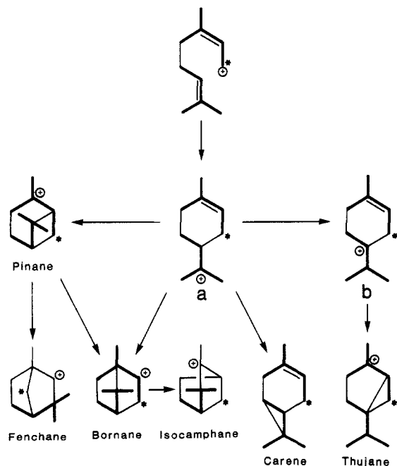
Figure 1. Representative monoterpenes.
